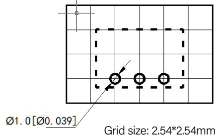
PCB Printing Layout
