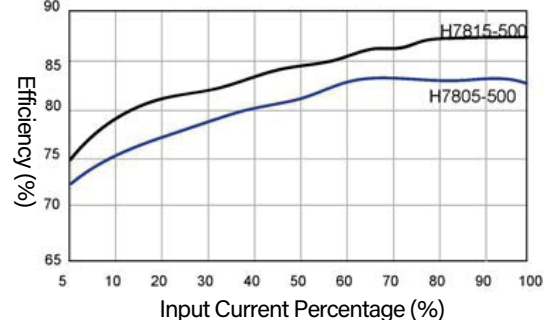
Negative Output Efficiency VS Output Load (Nominal Input)
