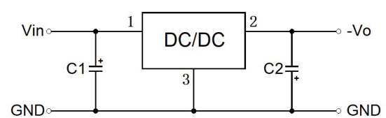
Figure 2-2 Negative output application circuit
