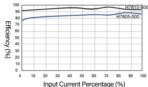
Positive Output Efficiency VS Output Load (Nominal Input)
